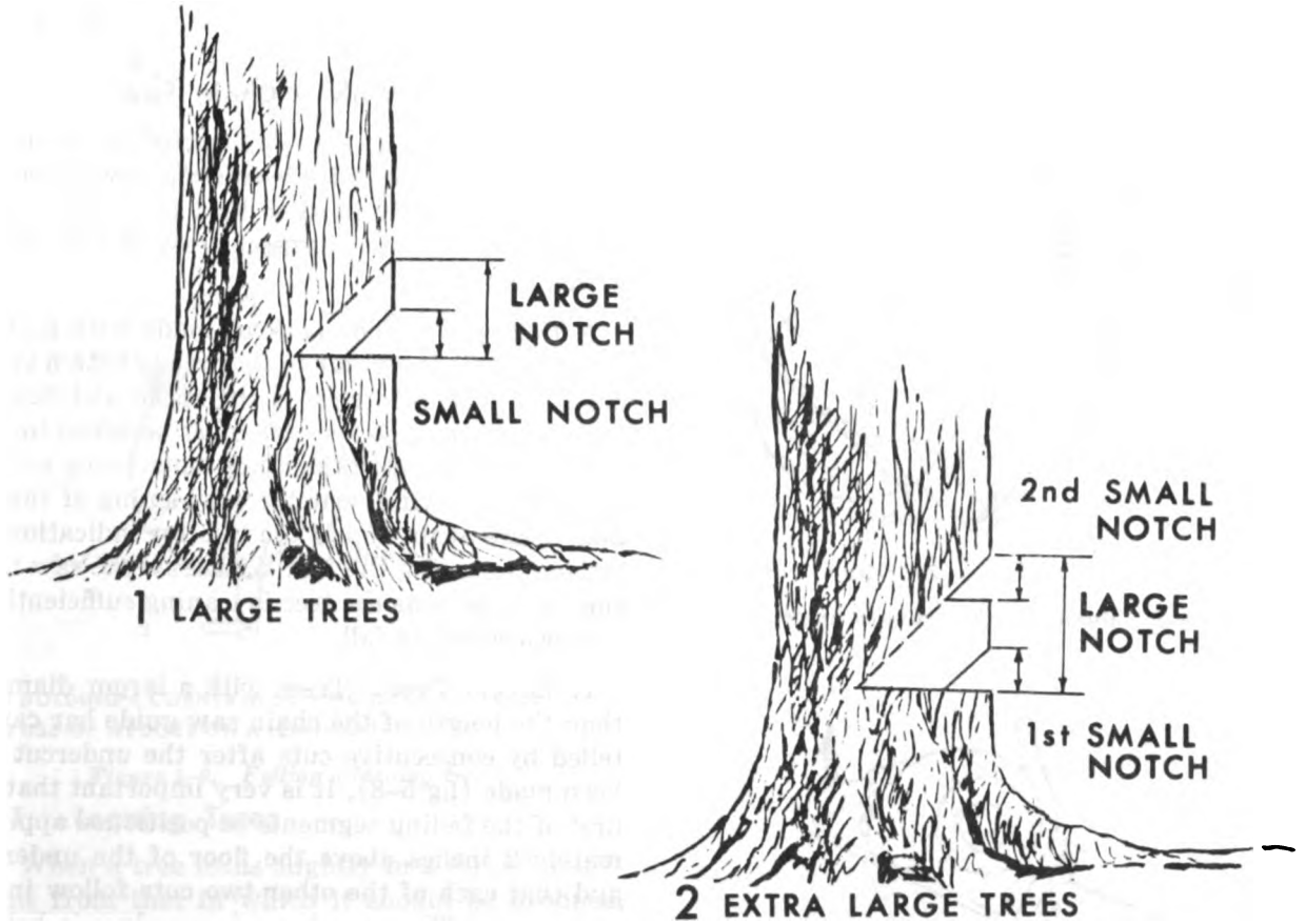
Figure 5-4. Notching a large tree.
